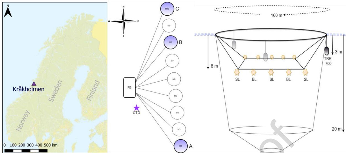
Figure 1. Location of the salmon farm Kråkholmen in central Norway (left panel), placement of the experimental cages A, B and C (middle panel) and the setup of underwater lights (right panel). CTDO-profiles were collected at a fixed point indicated by the blue star near the feeding barge (FB, middle panel). Ten lamps were submerged to eight-meter depth in two parallel rows approximately 12 meters apart, spanning the cage from east to west (SL=SubLite, BL=BlueLED, TBR700=Receiver).
