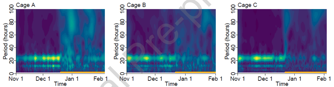
Figure 5. Wavelet spectra for all tagged fish in cages A, B and C, respectively. The orange horizontal lines represent the onset of underwater lights. Lights were activated on the 20 th December for cage A, and on the 22 nd of December for cages B and C.
