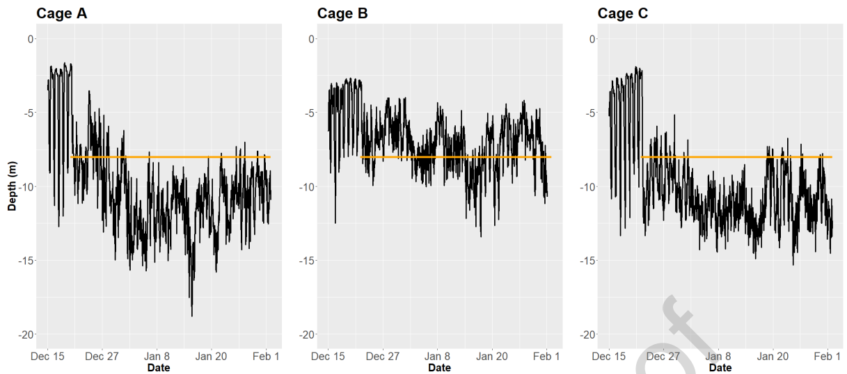
Figure 4. Average swimming depth for all tagged fish in the three cages from 15 th December - 2 nd February. The orange horizontal lines illustrate the depth and presence of artificial underwater lights.
